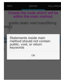
Figure 8. Prompt
