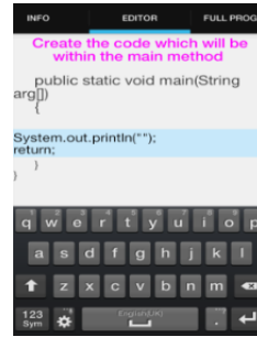
Figure 7. Main method
