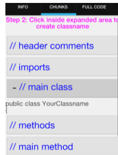
Figure 2. Default code
