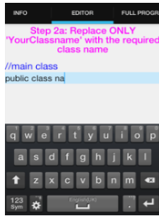
Figure 5. Main class
