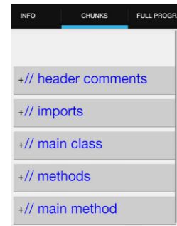
Figure 4. Unrestricted
