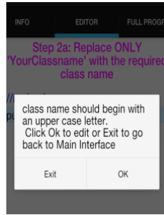
Figure 6. Prompt
