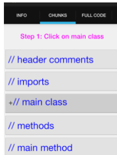
Figure 1. Main interface
